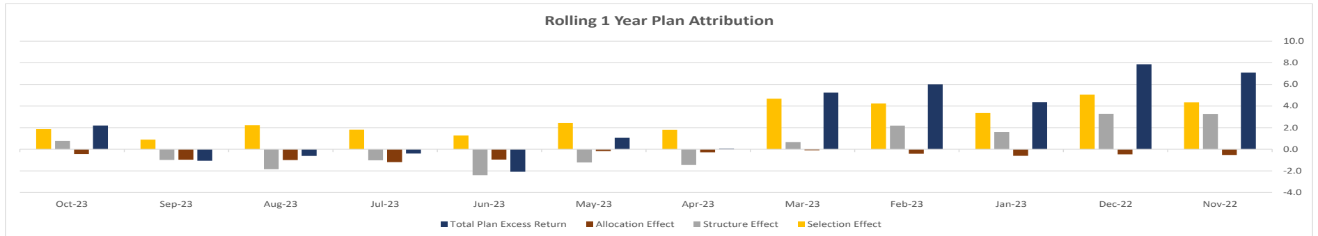
Selection Effect
